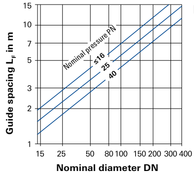
Recommended spacing for pipe guides in pipelines with axial expansion joints
